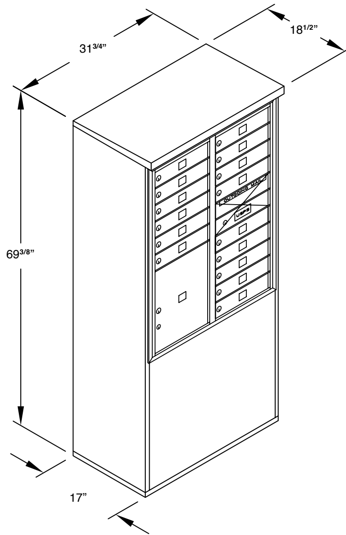
MODEL #3911D-15 - FRONT LOADING
