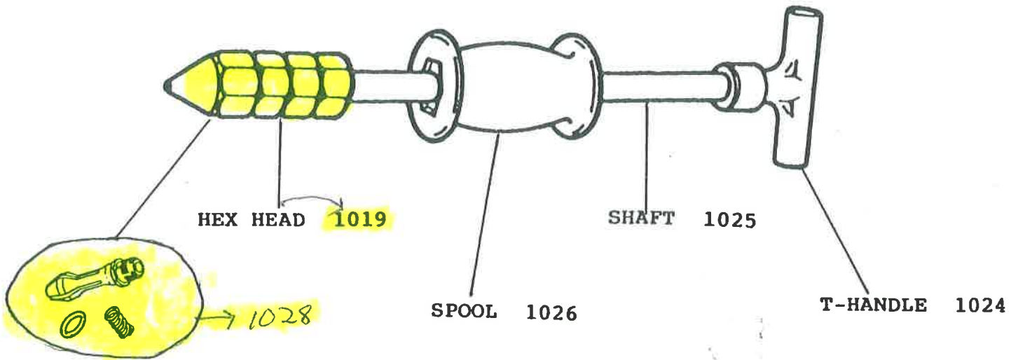
INSIDE HEX HEAD UNI-PULLER SERVICE KIT 1028
