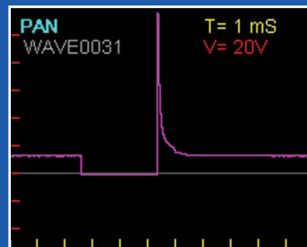
Injector snapshot
