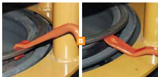
Mount end is used to mount split ring
