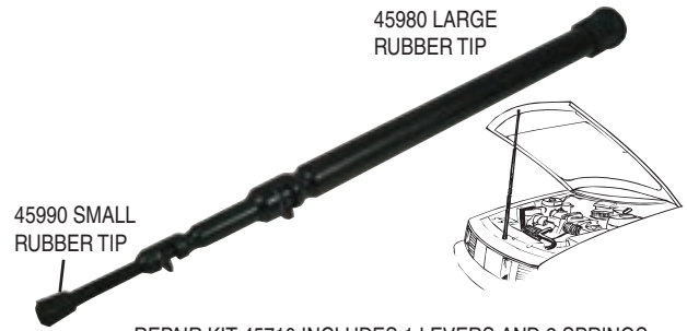
REPAIR KIT 45710 INCLUDES 1 LEVERS AND 2 SPRINGS
