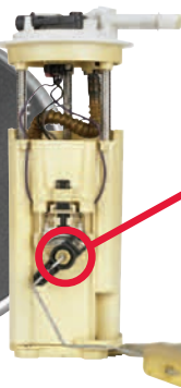
Damaged Worn, broken contacts cause inaccurate readings.
