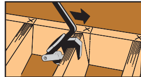
Straighten Joists.
