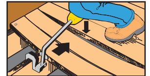
Hook Tool on Joist. Push Handle Down. Boards Squeeze Tight.
