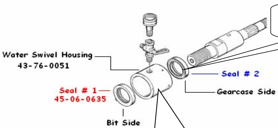
Water Swivel Housing 43-76-0051
