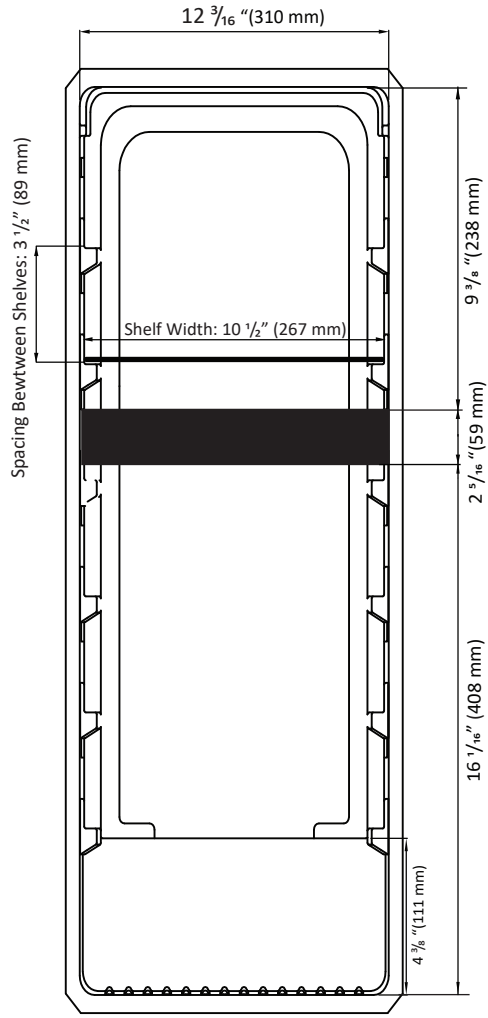
Front View
