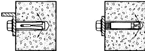
split sleeve and wedge anchors limited ring-shaped holding area
