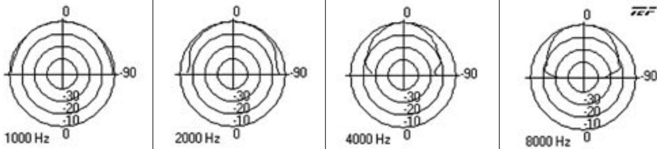
FAP42T Polars
