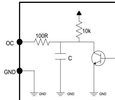
Figure 10: Over Current monitor pin interface
