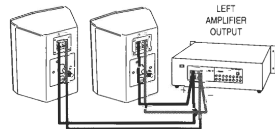
TYPICAL DAISY CHAIN CONFIGURATION
