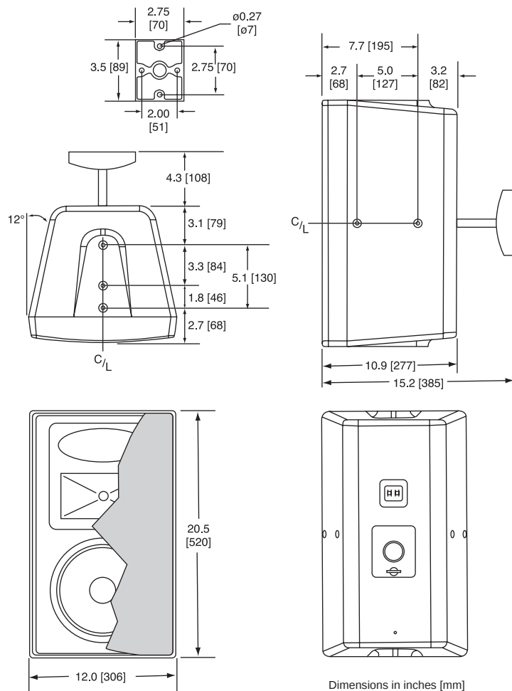
Dimensions in inches [mm]
