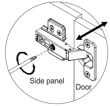
ADJUSTMENT GAP
