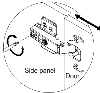
ADJUSTMENT DEPTH
