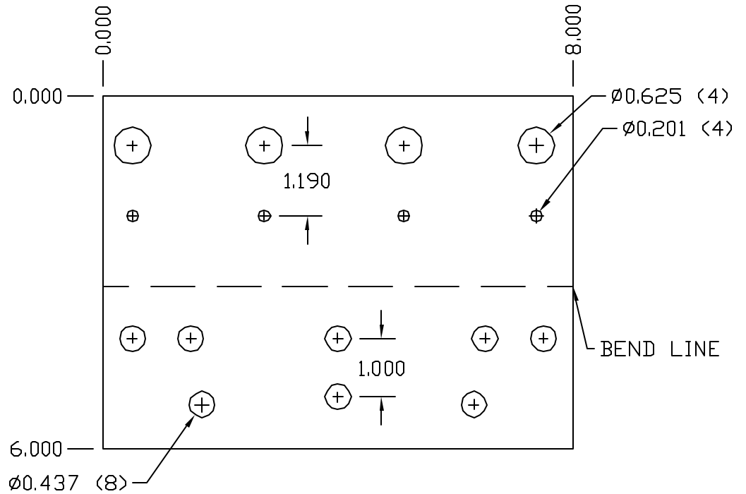
FLAT BAR LAYOUT
