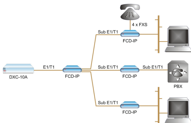
Figure 2. Aggregating Three Fractional E1 Links into One Full E1 Link
