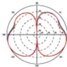
Vertical Radiation Pattern @ 2.4 – 2.5GHz
