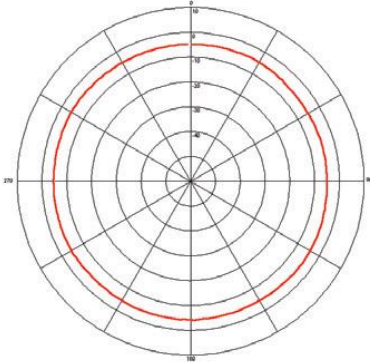
Azimuth Cut, Phi=0°
