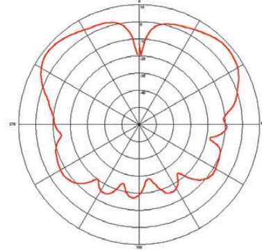
Elevation Cut, Phi=90°
