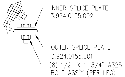
SECTION A-A SPLICE DETAIL #4
