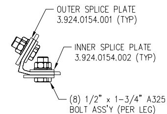
SPLICE DETAIL #3 SECTION B-B
