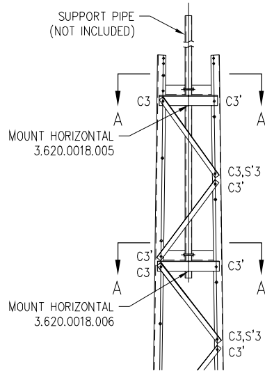
TOP SECTION #3 (INCLUDES ALL PARTS SHOWN IN SECTION #3)
