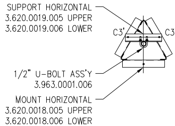
SUPPORT INSTALLATION SECTION A-A
