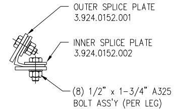
SPlice DETAIL #1 SECTION B-B
