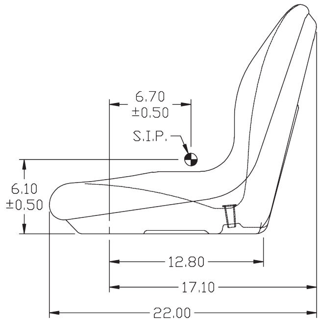
SEAT SIDE VIEW (OF SEAT THAT COVER FITS)
