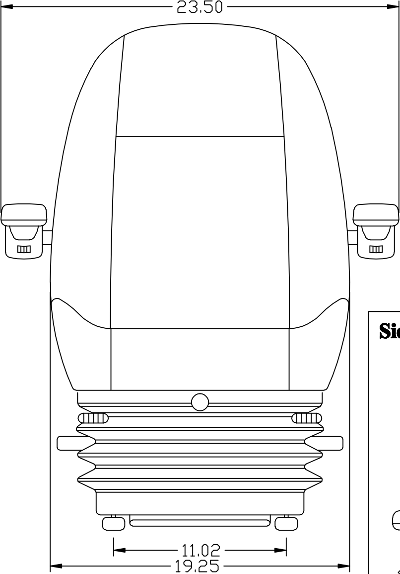
Front View
