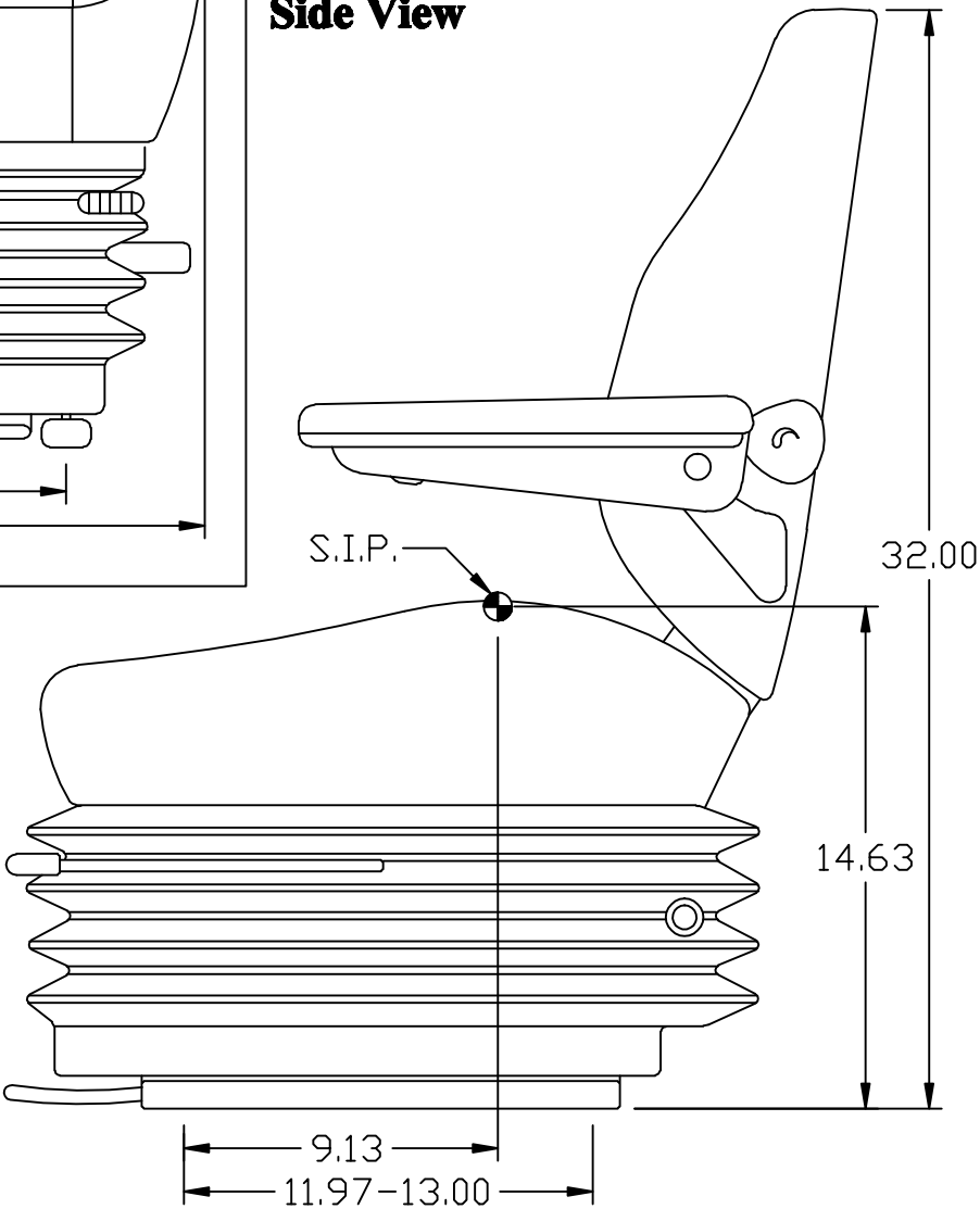
Side View
