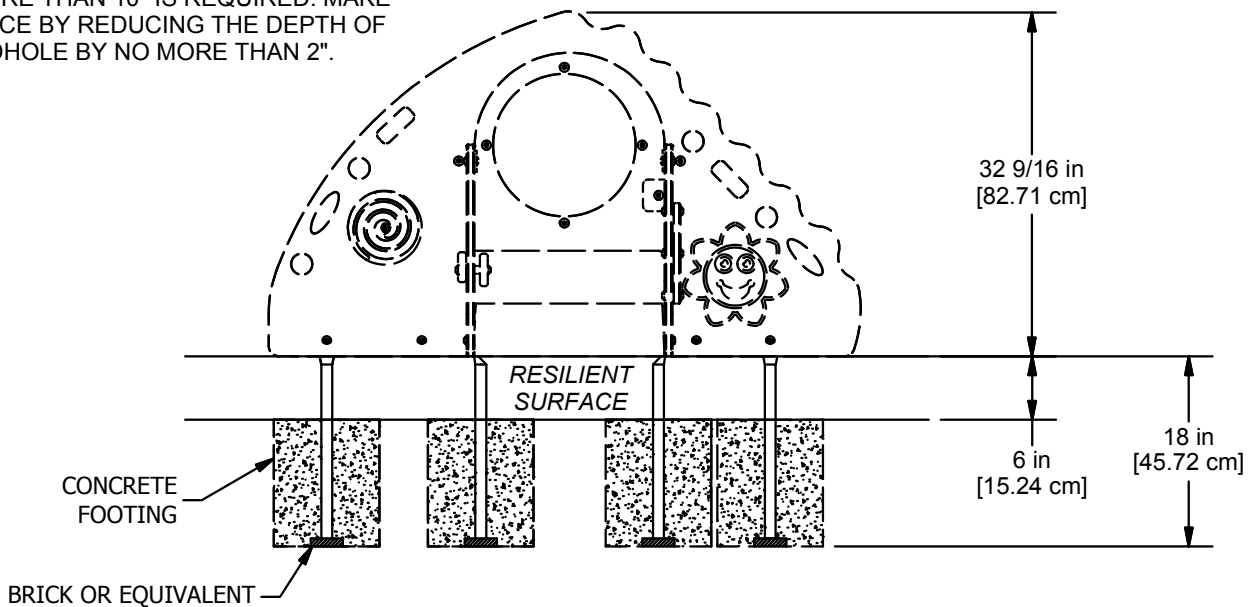
ELEVATION VIEW
