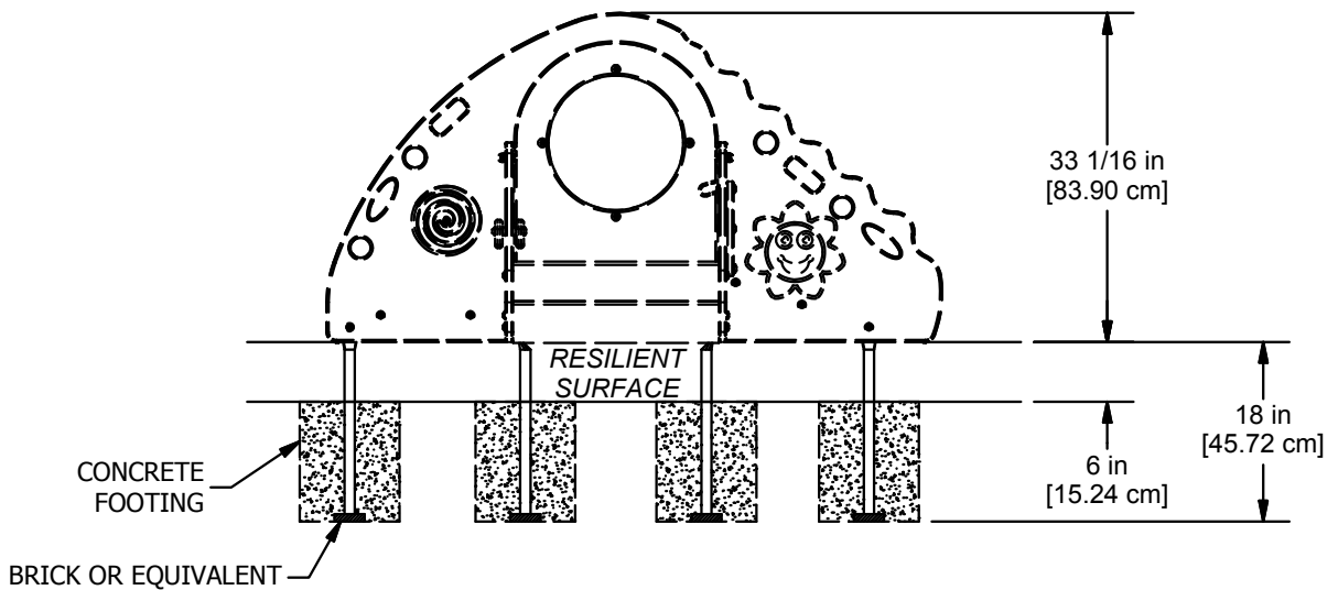
ELEVATION VIEW
