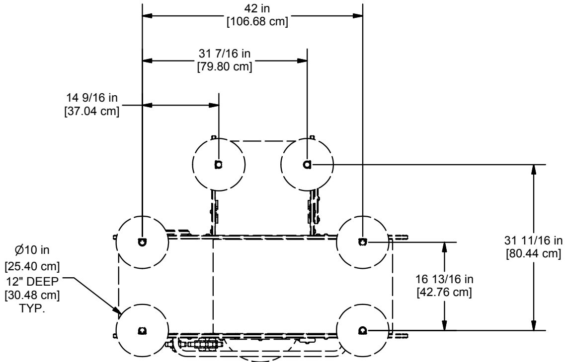
BOTTOM VIEW
