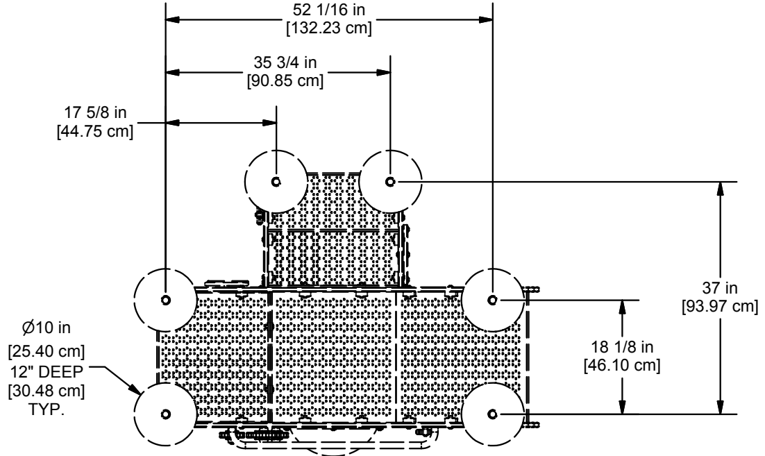
BOTTOM VIEW
